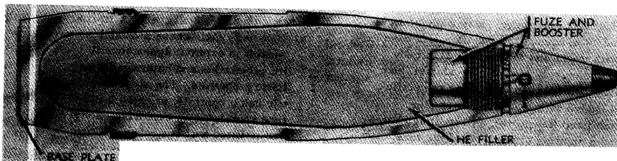
Fig 1-1 TYPICAL HE (HIGH-EXPLOSIVE) PROJECTILE W/O TRACER
